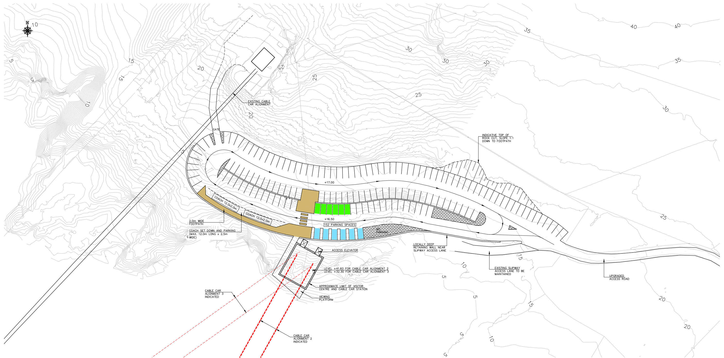
OPTION 2A AND 2B – MAINLAND SITE LAYOUT PLAN
